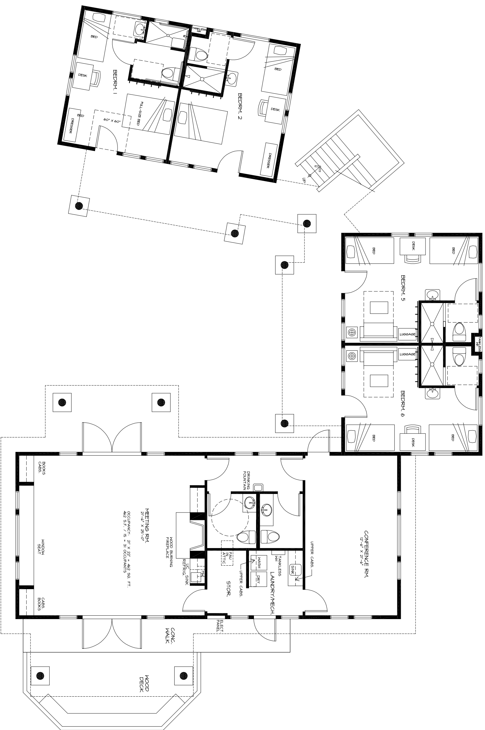
BERESTROM LODGE FIRST FLOOR PLAN 2305 S.F.
